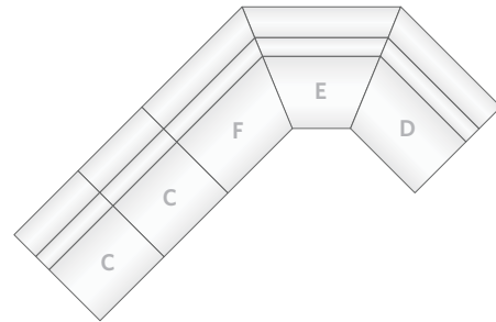
HALF RACETRACK
