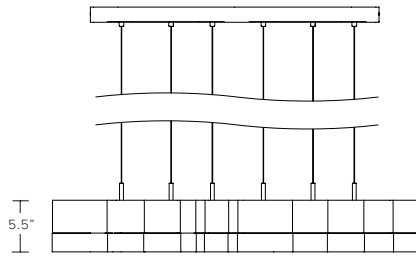
MULTI-MODULE CHANDELIER, 7 + 7
