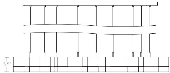
MULTI-MODULE CHANDELIER, 5+7+11
